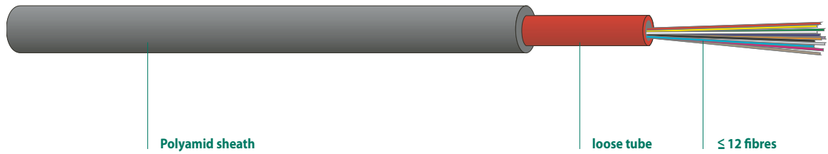
Polyamid sheath
